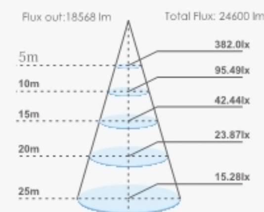
FL16 Illumination curve
