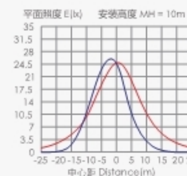
LD6A-1 Illumination curve
