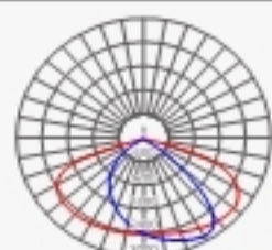
TYPE-1-SERIES 80°*150°
