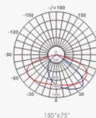
LD6A-1 Light distribution curve
