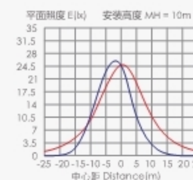
LD6A-1 Illumination curve
