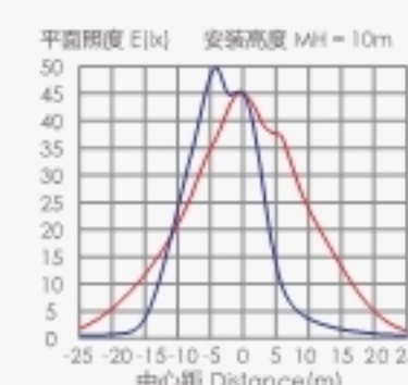
Illumination curve
