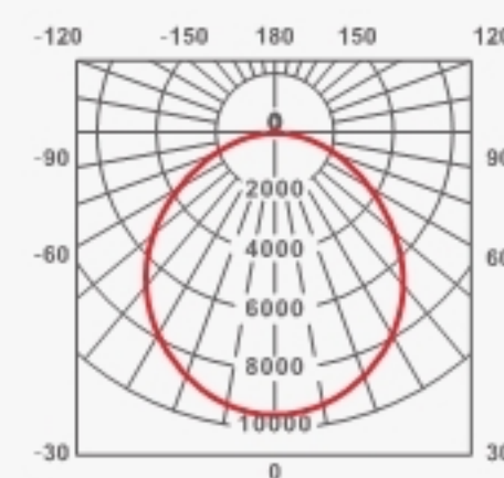
FL16 Light distribution curve
