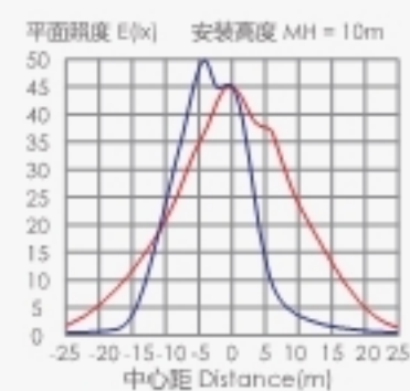
Illumination curve
