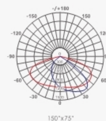
LD6A-1 Light distribution curve
