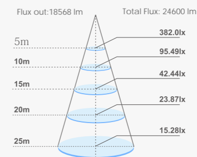
FL16 Illumination curve
