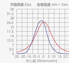
LD6A-1 Illumination curve
