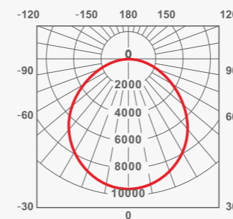
FL16 Light distribution curve
