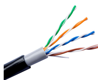
室外超五类非屏蔽阻水网线 Outdoor UTP Cat5e
