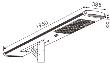
MODEL: WSL-100G2 | mm MODEL: WSL-120G2 | mm
