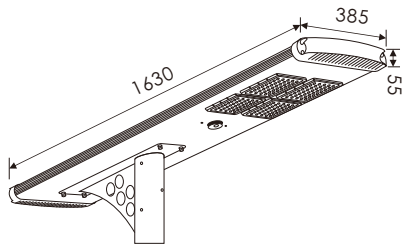
MODEL: WSL-80G2 | mm
