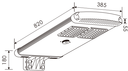
MODEL: WSL-30G2 | mm
