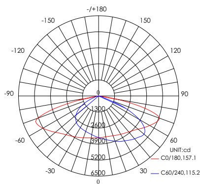
AVERAGE BEAM ANGLE(50%):135.5 DEG
