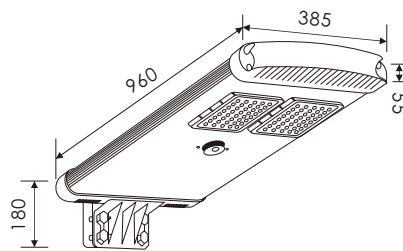
MODEL: WSL-40G2 | mm
