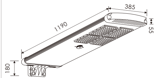
MODEL: WSL-50G2 | mm MODEL: WSL-60G2 | mm
