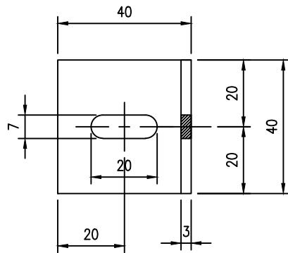
50x40x3 Aluminum Angle
