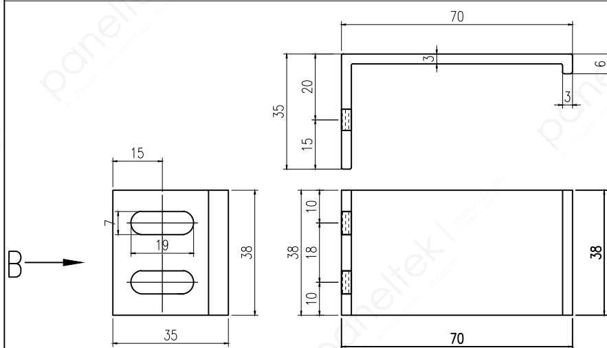
Elevation Drawing
