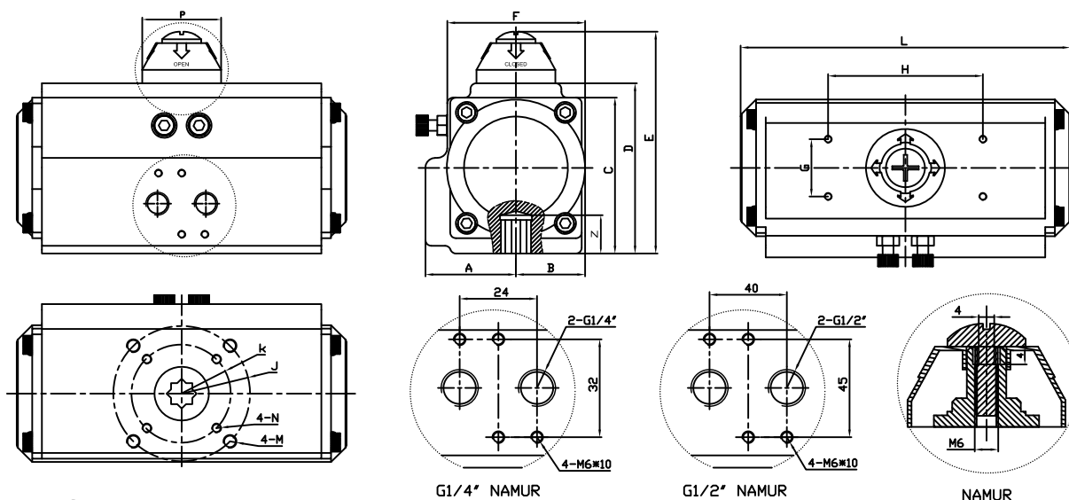
Outline Size drawing
